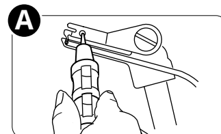
Rear view of the upper looper
