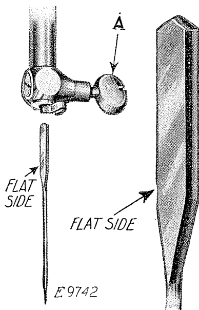
FIG. 11. POSITIONING OF NEEDLE IN NEEDLE CLAMP
