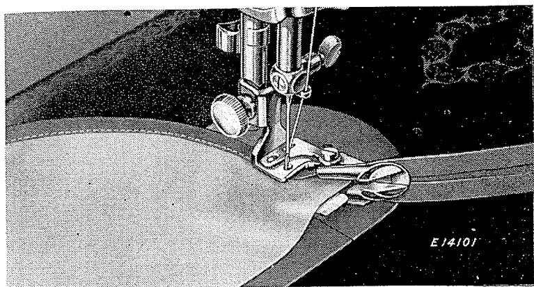
FIG. 44. BINDING AN OUTSIDE CURVE
