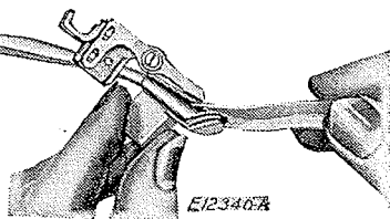
FIG. 42. INSERT FOLDED BINDING IN OUTSIDE SLOT
