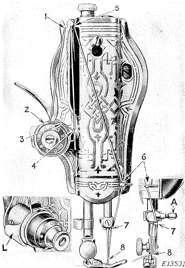
FIG. 12. UPPER THREADING
