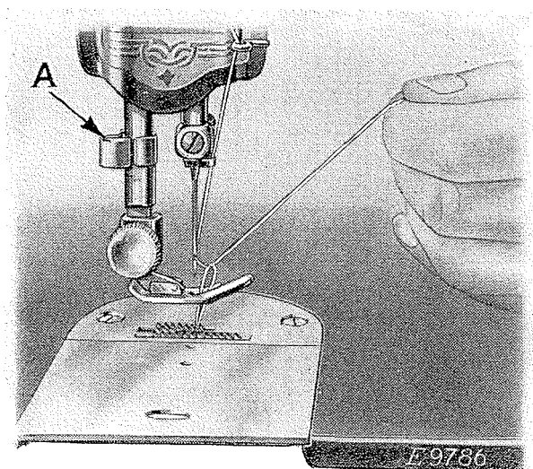
FIG. 13. DRAWING UP THE BOBBIN THREAD
